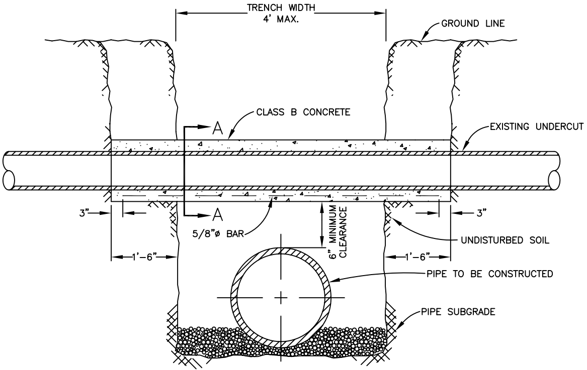
TYPICAL SECTION
