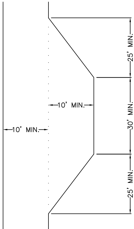
TURNOUT DETAIL 1
